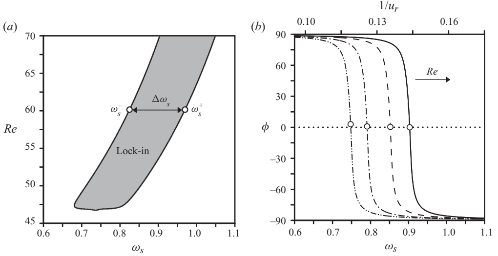
FIGURE 7. Effect of the natural frequency \omega_s for \gamma = 0.01 and m = 10\,000 . (a) Boundary of the resonance width \Delta\omega_s as a function of the Reynolds number. The inner grey shade therefore defines the lock-in state. (b) Phase shift \phi as a function of \omega_s for the same Reynolds numbers as in figure 6(b). The circles denote the value \phi(\omega_s^{max}) at lock-in.
