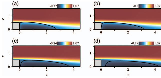
FIG. 12. (Color) Spatial distribution of streamwise velocity for the nonlinearly forced base flow \mathbf{Q}_w , obtained by solving directly the homogeneous form of the nonlinear base flow equations (11) along with the additional condition \mathbf{U} = \delta W_w \mathbf{e}_z at the base— \text{Re} = 2000 , M = 0.5 . (a) \delta W_w = 0.001 , (b) \delta W_w = 0.02 , (c) \delta W_w = 0.04 , and (d) \delta W_w = 0.06 .
