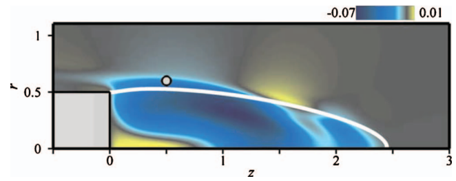
FIG. 7. (Color) Growth rate variation \delta\sigma(r_c, z_c) induced by a localized heat source modeled by Eq. (31) with \alpha=10^{-2} — \text{Re}=999 , M=0.5 . The circle symbol at (r_c, z_c)=(0.6, 0.5) indicates the position for which the sensitivity analysis to base flow modifications is carried out.
