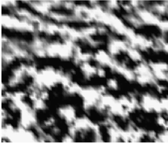
Fig. 12. Curl of the topos (spatial eigenvector) number 15.
