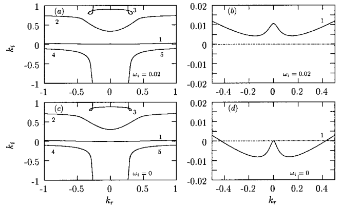
FIG. 2. Spatial branches k_n in the (k_r, k_i) plane for dispersion relation (19) with \omega_i = 0.02 (top) and \omega_i = 0.0 (bottom). R=40 , \beta=4.6^\circ , W=41.46 ( \Gamma=769.8 ). Left: overall view of the diagram. Right: zoom on the neighborhood of the origin in the complex k plane.
