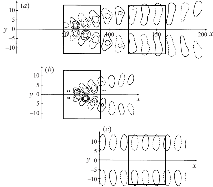
FIGURE 21. Interpretation of global mode structure (a) in terms of a front (b) and fully nonlinear travelling waves (c). Isopleths of fundamental streamwise velocity component are shown (0.05, 0.10, 0.15 solid lines, -0.05 , -0.10 , -0.15 dashed lines).
