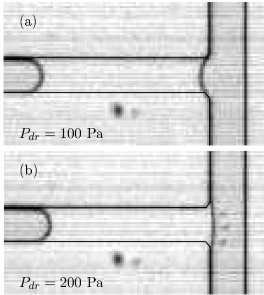
Figure 6. Blocking of the plug at the entrance of the T-junction for two distinct pressures with P_{dr} < P_{thresh} . The front interface is pinned at the corners of the bifurcation and adapts its in-plane curvature to the applied pressure. The shape of the rear interface is independent of P_{dr} .
