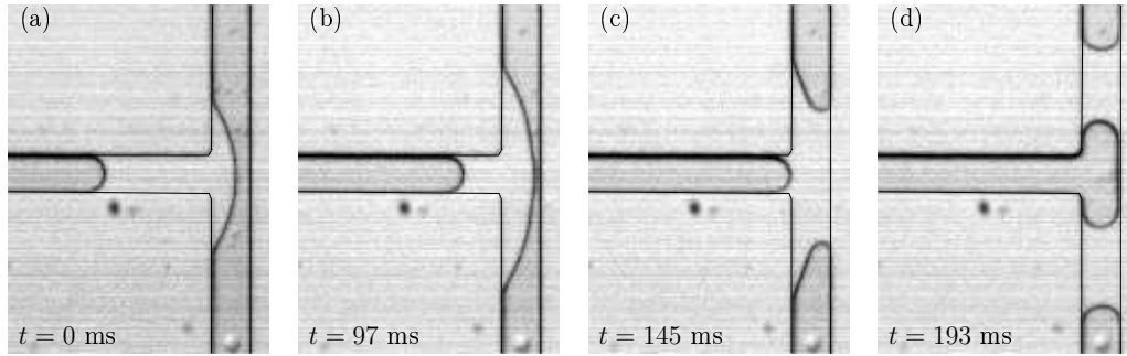
Figure 8. Sequence of plug splitting at the T-junction. Splitting leads to symmetric formation of two daughter plugs in the outlet branches of the T-junction.
