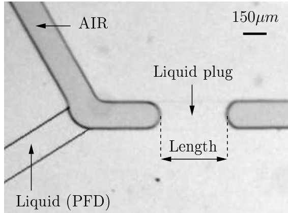
Figure 2. A liquid plug after its formation within the Y-junction. The plug moves from left to right. The upper branch is connected to the constant pressure source (air) and the lower branch contains the wetting liquid which is injected using a syringe pump. Length and speed are calculated from the measured positions of the menisci at the advancing (front) and receding (rear) interfaces, detected along the centerline of the channel.
