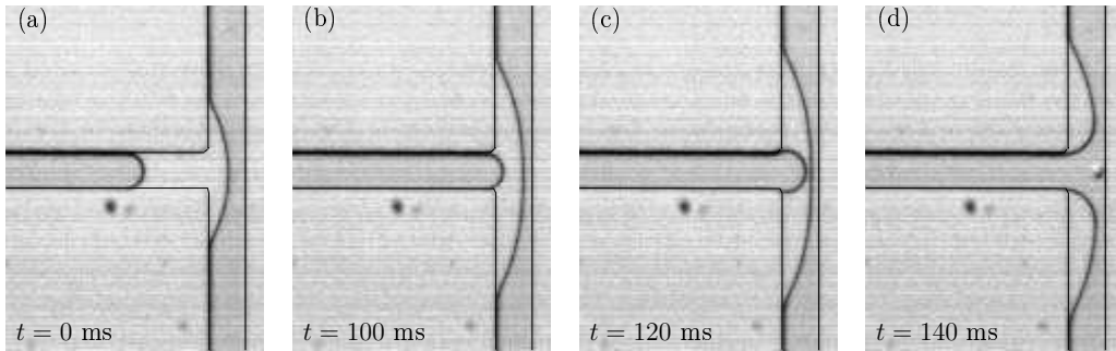
Figure 7. Sequence of plug rupture. The plug ruptures in the T-junction, leaving liquid on one side of the outlet channel, where air can flow freely from the pressure source.
