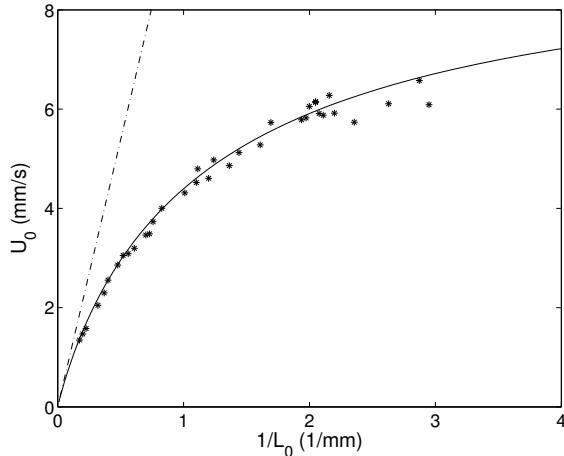
Figure 5. Average speed U_0 of a liquid plug as a function of its inverse length L_0^{-1} for a pressure P_{dr} = 250 Pa. The dotted line corresponds to Poiseuille's law, U_0 \propto L_0^{-1} . The full line corresponds to Eq. 10 with \beta = 16 .
