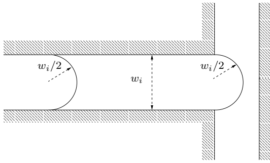
Figure 10. The shapes of the rear and front interfaces at the threshold pressure (in-plane section).
