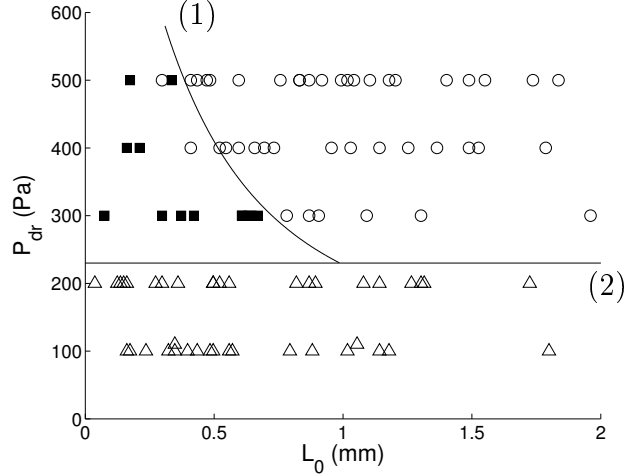
Figure 12. Experimental P_{dr} - L_0 diagram and theoretical transitions. (1)-Rupture-splitting transition corresponding to Eq. 23 with \theta^a varying from 0 to \pi/3 and (6\Gamma)^{1/3} = 4.9 . (2)-Threshold pressure (Eq. 13).
