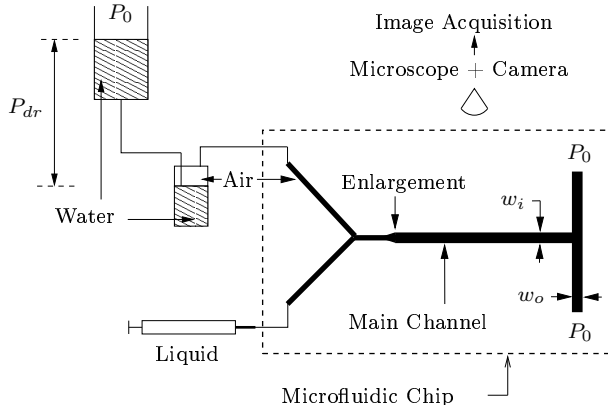
Figure 1. Experimental setup. A constant pressure P_{dr} is applied at the upper left inlet branch of the Y-junction. The lower left branch is used to introduce the wetting liquid from a syringe pump. The motion of the plug is recorded with a camera through a microscope. Note the enlargement of the inlet channel downstream of the Y-junction.
