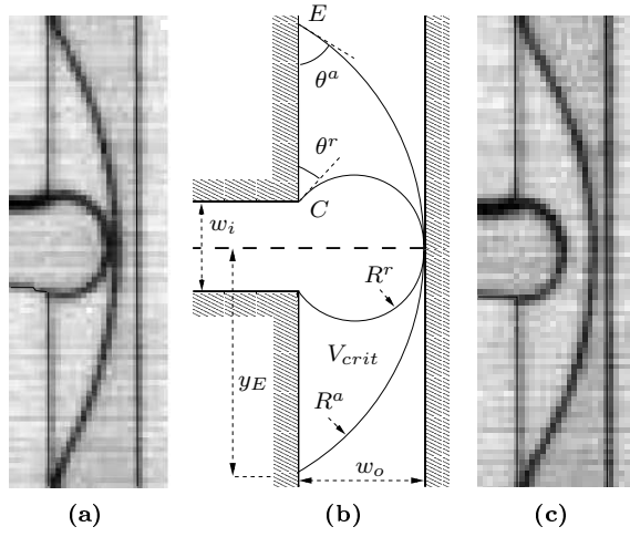
Figure 11. Shape of the plugs before (a) -rupture and (c) -splitting. - (b) Schematic of a plug of volume V_{crit} situated on the theoretical boundary between rupture and splitting where front and rear interfaces of a plug meet at the wall.
