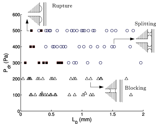
Figure 9. Phase diagram for plug behavior at the T-junction.
