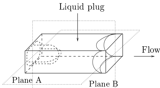
Figure 3. Schematic of a plug in a rectangular channel. Planes A and B correspond respectively to “in-plane” and “in-thickness” sections.
