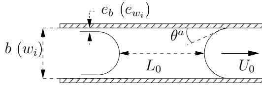
Figure 4. Plug geometry: \theta^a is the dynamic contact angle at the front interface and e_b (e_{w_i}) is the thickness of the deposited film at the rear of the plug in the thickness (width).
