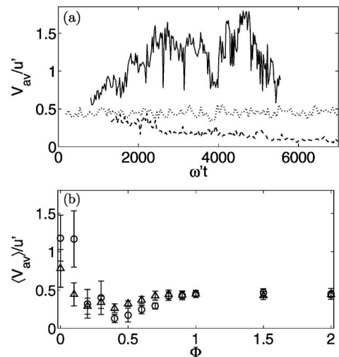
FIG. 5. (a) Temporal evolution of the vortex mobility. n=1 , Re=7000 . \Phi=0 (—); (---) 0.5; (·····) 1.0. (b) Mean vortex mobility vs \Phi . n=1 . ( \Delta ) Re=1400 ; ( \circ ) Re=7000 .
