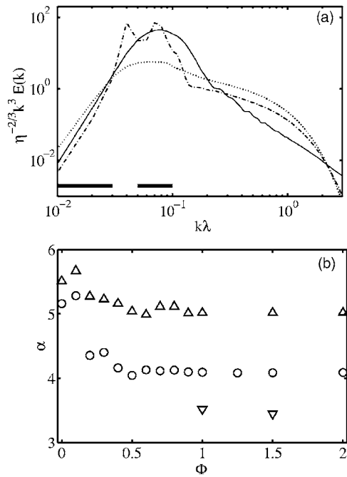
FIG. 1. (a) Enstrophy spectral density, k^3 E(k) , in viscous units. n=1 , Re=7000 . \Phi=0 (—); (---) 0.5; ( \cdots ) 1.0. The two horizontal segments are the ranges for forcing and for low-wavenumber damping. (b) Slope of the energy spectrum. ( \Delta ) n=1 , Re=1400 ; ( \circ ) n=1 , Re=7000 ; ( \nabla ) n=4 , Re=12\,500 .
