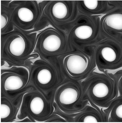
FIG. 4. Vorticity for \Phi=0.5 . The coherent vortices are, in this case, positive. Other parameters as in Fig. 2.
