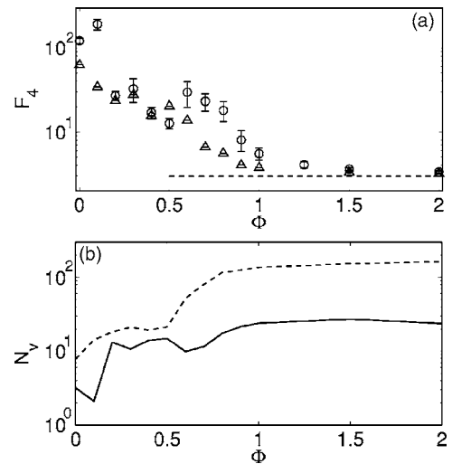
FIG. 3. (a) Fourth-order flatness of the vorticity as a function of \Phi . (----) Gaussian. Error bars are one \sigma . n=1 . ( \Delta ) Re=1400 ; ( \circ ) Re=7000 . (b) Number of coherent vortices. (—) D > L/2 ; (----) all vortices. n=1 , Re=7000 .
