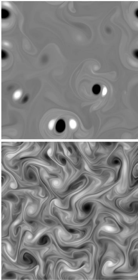
FIG. 2. Vorticity. (Top) \Phi=0 . (Bottom) \Phi=1.5 . The grayscale spans in both cases the range \pm 4\omega' . n=1 , Re=7000 .
