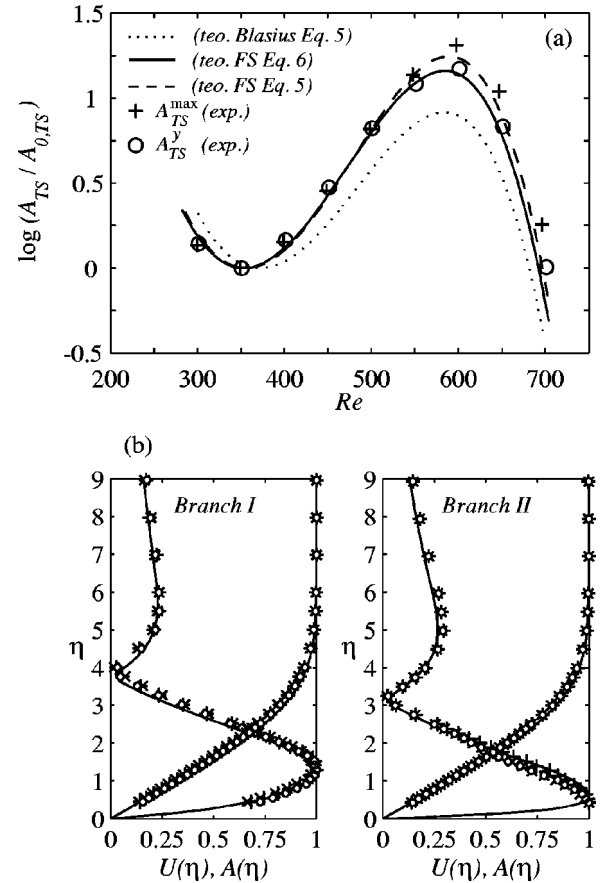
FIG. 20. (a) TS amplification curves of the R case. (b) Shows the wall-normal mean ( U ) and TS amplitude ( A ) profiles for three different spanwise positions (+, \times , \circ ) close to branches I ( \text{Re}=351 ) and II ( \text{Re}=601 ). Solid lines are the theoretical FS profiles with m = -0.0046 . F = 130 .
