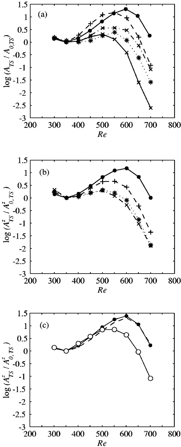
FIG. 18. Alternative amplitude measures. (a) shows the maximum measure, (b) the y-integral measure, and (c) the z-integral measure. The different symbols correspond to R case ( \bullet ); S_2 case (+) high speed, (*) shear, ( \times ) low speed, and ( \circ ) the spanwise integrated. Dash-dotted and solid lines of ( \times ) correspond to outer and inner peaks, respectively, and other lines are for visual aid only. See text for dashed line in (c). F=130 .
