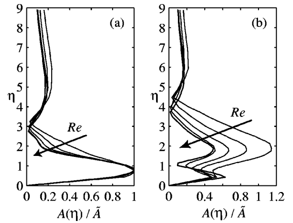
FIG. 11. Wall-normal amplitude profile evolution for F=110 . (a) High- and (b) low-speed location. Re=451, 501, 551, 601, 651 . \tilde{A} corresponds to the inner peak value in the high-speed location for each Re .
