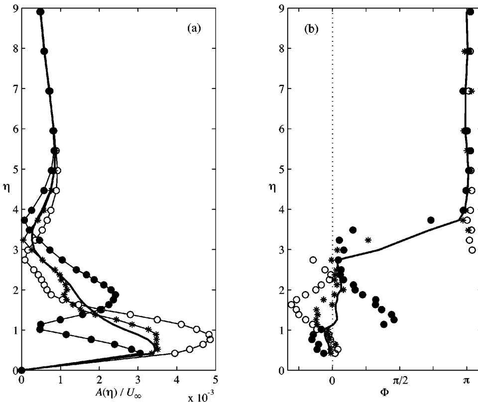
FIG. 10. (a) Wall-normal TS amplitude profiles and (b) corresponding phase distributions of Fig. 9. ( \circ ), ( \bullet ), and ( * ) correspond to the high-, the low-, and the shear-speed spanwise locations. Bold solid line correspond to the spanwise averaged profile. F=110 and Re=651 .
