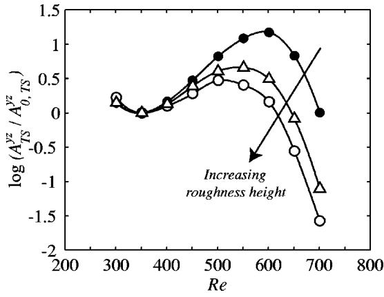
FIG. 14. TS amplification curves for the R case (●) and for successively increasing roughness heights S_1 and S_2 (△,○). F=130 . Solid lines are fitted spline curves to the experimental data.
