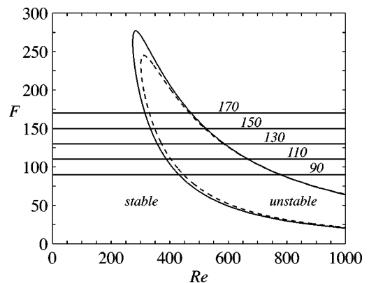
FIG. 8. Neutral stability curves for the FS (solid line), with m=-0.0046 , and the Blasius boundary layers (dashed line). The horizontal lines indicate the five frequencies studied in the present investigation.
