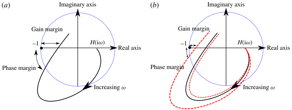
FIGURE 4. (Colour online) Nyquist plot of the OLTF, showing phase and gain margins, based on the nominal system (a) and the nominal system with uncertainty bounds (b).
