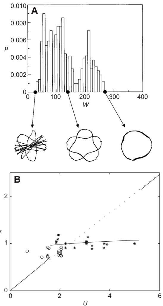
Fig. 8. Taking into account the variability in the properties of individual components. (A) The probability density function ( p ) of the wear work rate ( W , the product of the impact force by the sliding velocity) following a large number of simulations of tube motions, in a Monte-Carlo approach (Delaune et al., 2000). The probability density function shows a large variety of possible responses of the system. (B) A comparison between experimental (symbols) and model (line) of the local frequency ( f ) of oscillation of a crop canopy under flow, as a function of the flow velocity ( U ) (modified from Py et al., 2006). The model is based on the characteristics of the average plant.
