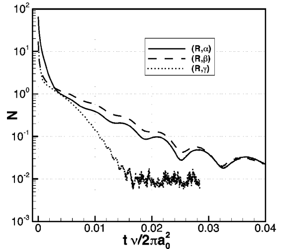
FIG. 2. Euler-residue N versus time scaled by the viscous time. Case (R).
