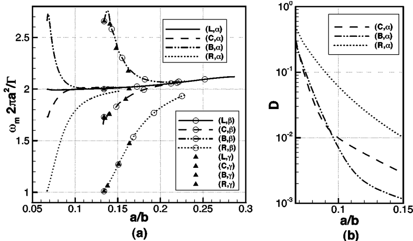
FIG. 5. (a) Peak vorticity \omega_m normalized by \Gamma and a versus the dipole aspect ratio a/b . (b) Deviation D between ( C, B, R ) simulations and ( L ) simulation versus a/b .
