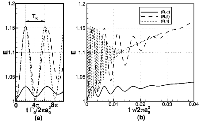
FIG. 1. Vortex aspect ratio E versus (a) time scaled by the advective time; (b) time scaled by the viscous time. Case (R).
