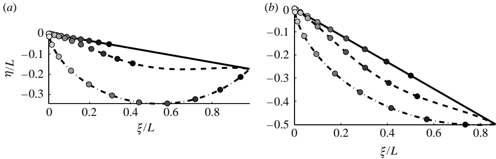
Figure 13. Predicted trajectories of a rolling point mass along a rigid ramp (solid line), a flexible beam (dashed curve, \mathcal{K}=1 , \mathcal{M}=3 ), and a brachistochrone curve (dash-dotted curve) for (a) \theta=10^\circ and (b) \theta=30^\circ . The shading denotes the positions at equal times, spaced by equal intervals \Delta\bar{t}=0.2 .
