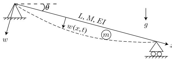
Figure 10. Schematic of a sphere with mass m traversing a simply supported inclined beam having length L , mass M , stiffness EI and initial inclination \theta . A particular beam deflection w(x, t) is shown.
